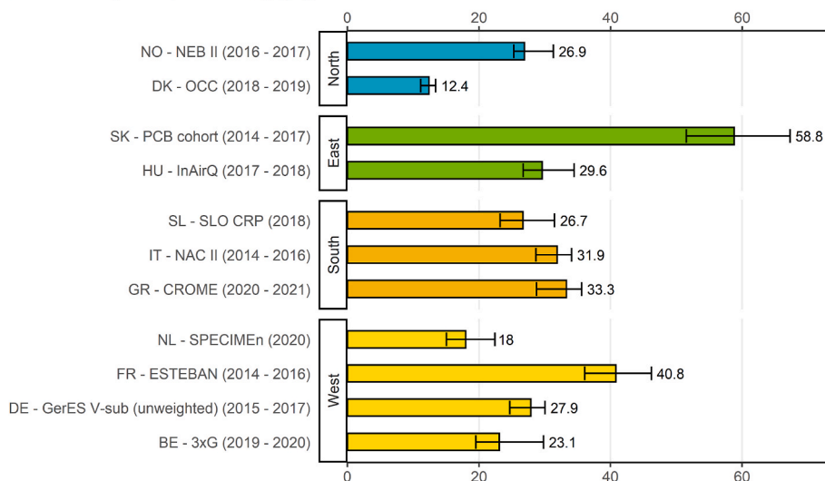
Fig. 2. Result indicator for geographical differences of P50 values (and 95% confidence intervals) in DiBP exposure (MiBP in \mu\text{g}/\text{l} ) in children (6–11 years) in the HBM4EU Aligned Studies. Country names, study names and sampling years (in brackets) are given. DiBP metabolite levels were either measured in first morning or random spot urine samples.
