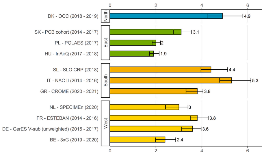
Fig. 3. Result indicator for geographical differences of P50 values (and 95% confidence intervals) for DINCH exposure ( \Sigma (OH-MINCH + cx-MINCH) in µg/L) in children (6–11 years) in the HBM4EU Aligned Studies (collected in the years 2014–2021). Country names, study names and sampling years (in brackets) are given. DINCH metabolite levels were either measured in first morning or random spot urine samples.
